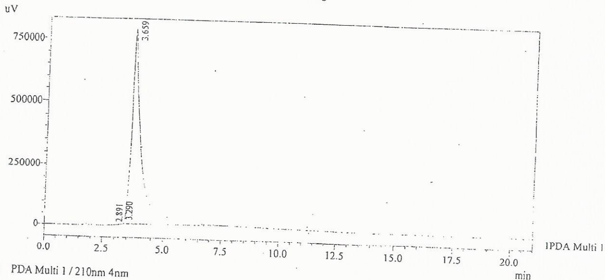
Chromatogram
